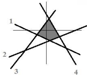
Figure 1. The convex feasibility problem
