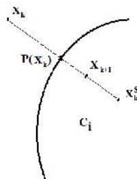
Figure 2. The projection algorithm
