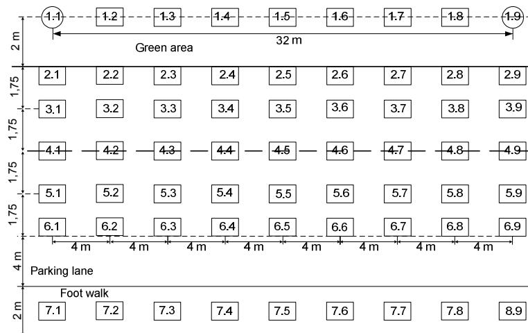
Figure 5. Measurement points for illumination and luminance levels.
