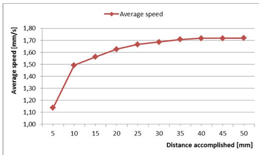
Figure 5. Translational joint average speed, depending on distance accomplished
