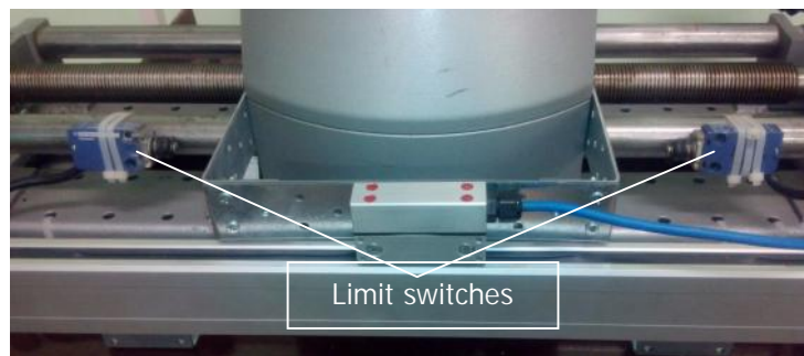
Figure 3. Limit switches mounted on the horizontal guiding columns [8]
