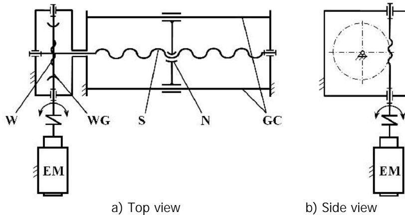
Figure 2. Kinematical scheme of the base mechanical transmissions [8]
