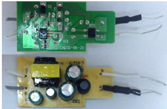
Figure 7 . PCB board of a measured LED lamp.
