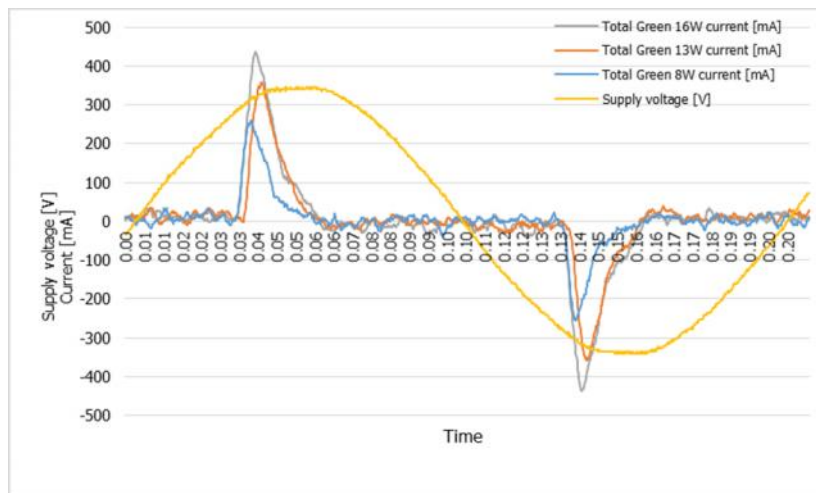
Figure 2. Total Green LED lamps current waveforms
