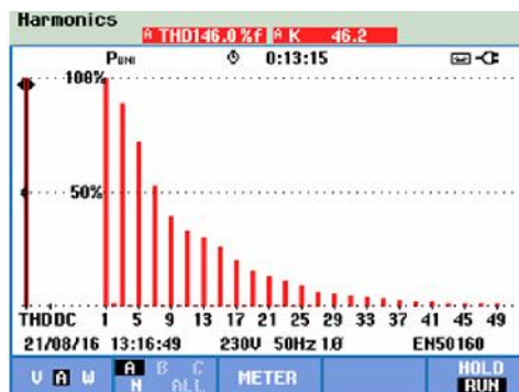
Figure 5. Total Green 13W LED lamp - (THDi=146 %, THDu=1.7 %).
