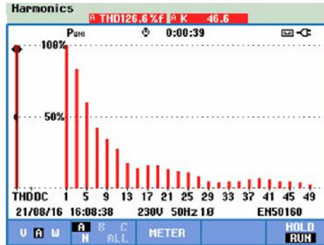
Figure 6. Philips 13.5W LED lamp - (THDi=126.6 %, THDu=1.1 %).
