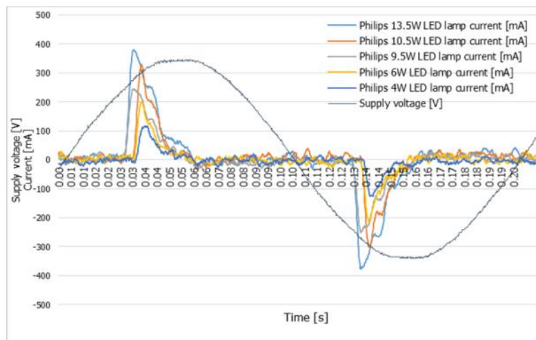
Figure 3. Philips LED lamps current waveforms
